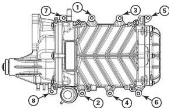
Supercharger bolt tightening sequence
