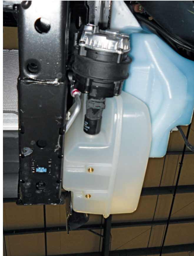
3. Install two (2) intercooler pump mounting brackets (1318-8C4191) (upper) over the frame as shown.
